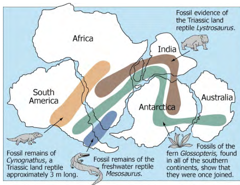
Figure 5.34. Fossil Evidence of Continental Drift
